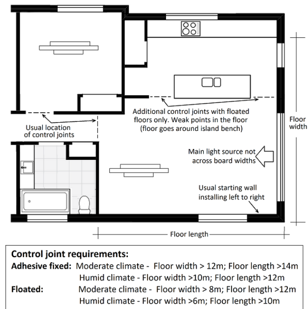
Figure 2 – Installation
