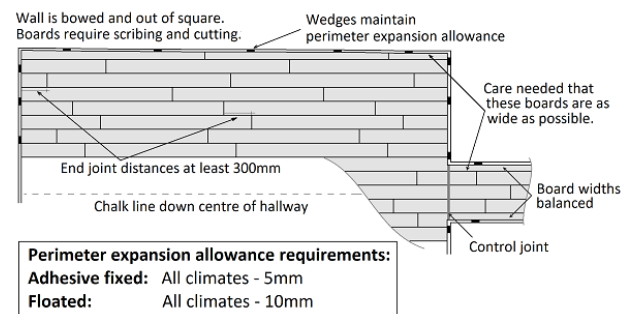
Figure 3 – Scribing
