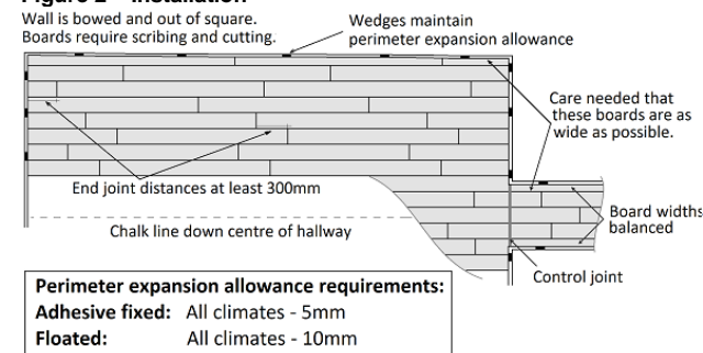
Figure 3 – Scribing
