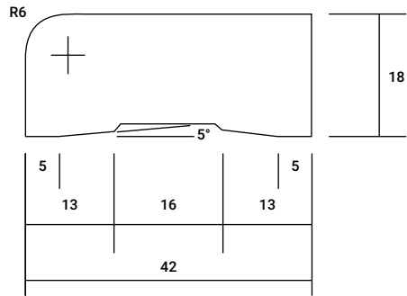
PENCIL ROUND AS7 42mm x 18mm
