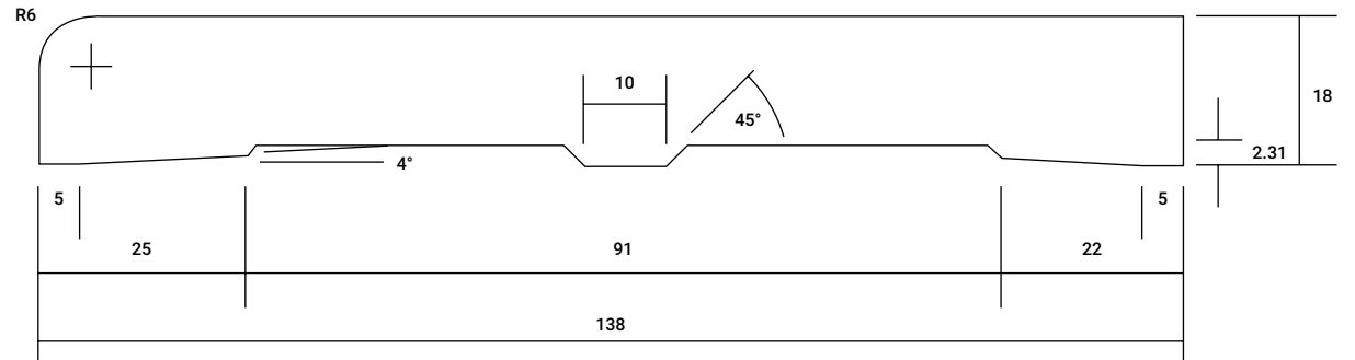
PENCIL ROUND AS7 138mm x 18mm
