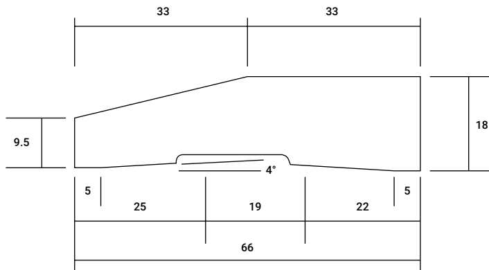
HALF SPLAYED AS5 66mm x 18mm
