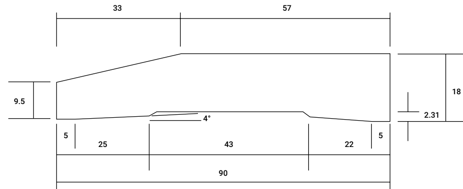
HALF SPLAYED AS5 90mm x 18mm
