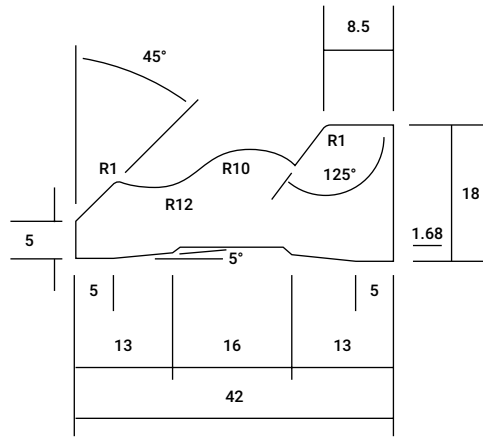
COLONIAL AS2 42mm x 18mm
