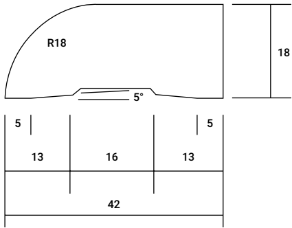
BULLNOSE AS1 42mm x 18mm
