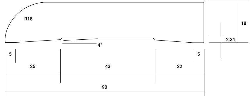
BULLNOSE AS1 90mm x 18mm
