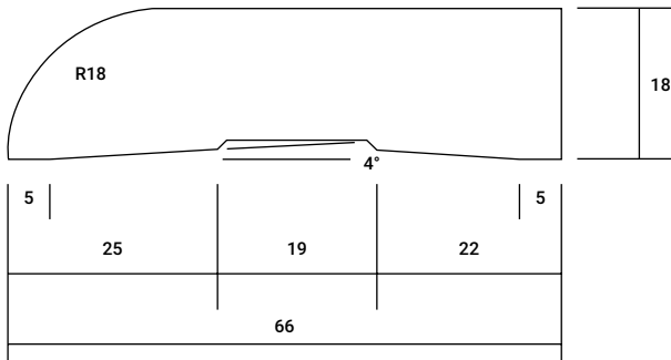
BULLNOSE AS1 66mm x 18mm
