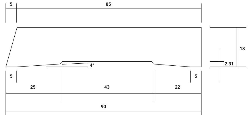
BEVEL AS3 90mm x 18mm
